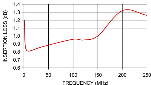
ADT9-1T INSERTION LOSS
